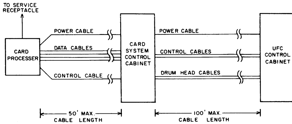
Figure 7-3. Cabling Diagram
