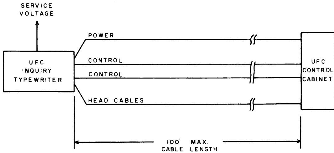
Figure 4-2. Cabling Diagram for Inquiry Typewriter
