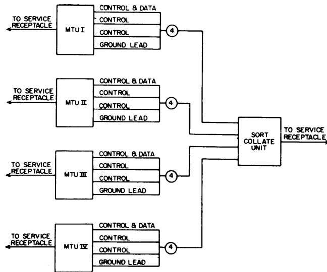
Figure 9-3. Cabling Diagram for Independent Operation of Sort-Collate System
