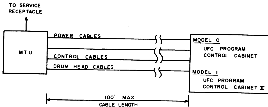
Figure 8-2. Cabling Diagram for Operation of Univac File-Computer Magnetic Tape Unit as I/O Unit
