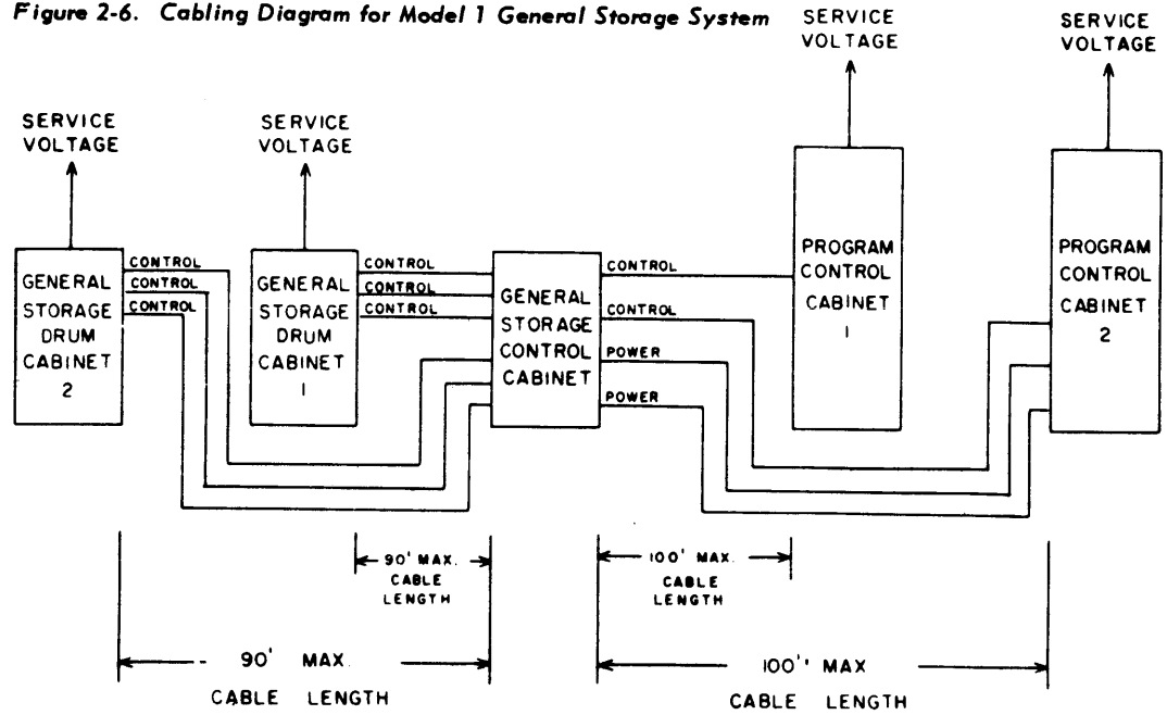
Figure 2-6. Cabling Diagram for Model 1 General Storage System
